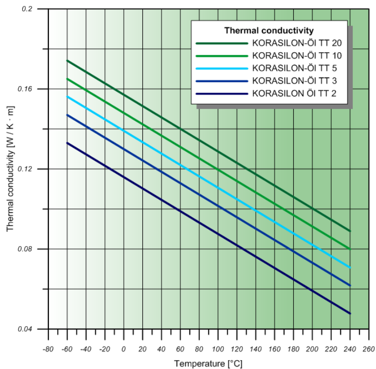
Thermal conductivity as function of temperature
